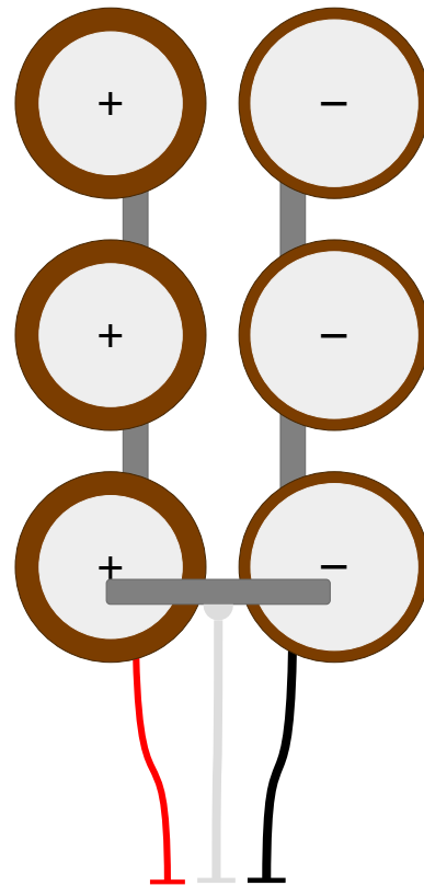
Bottom View
